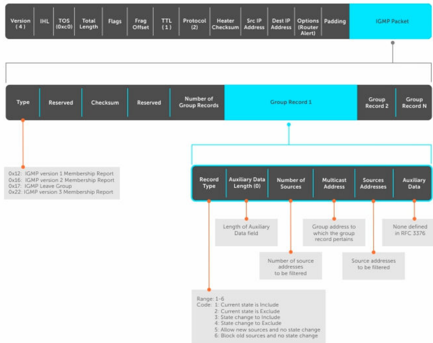
Figure 39. IGMP Version 3–Capable Multicast Routers Address Structure
